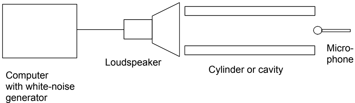
Figure 1. Schematic of the acoustics experiment, showing the computer, loudspeaker, cylinder or resonant cavity, and microphone. The output of the microphone is returned to the computer for processing.
